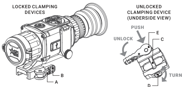
FIGURE 2-6. MOUNT
