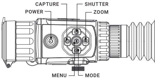
FIGURE 2-3. CONTROL BUTTONS
