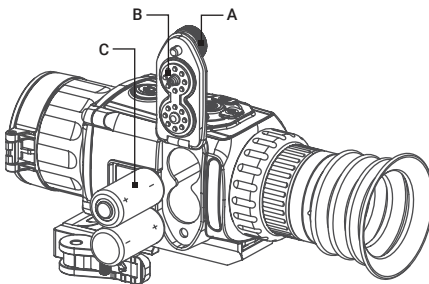
FIGURE 2-1. BATTERY INSTALLATION
