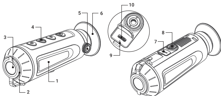
FIGURE 1-1. MAIN PARTS
