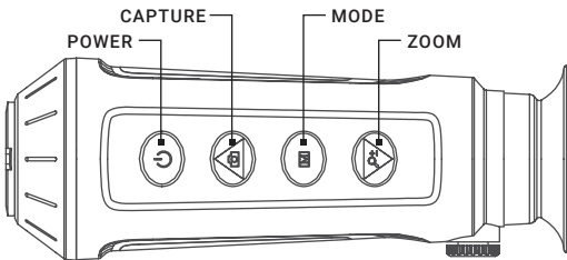
FIGURE 2-2. CONTROL BUTTONS
