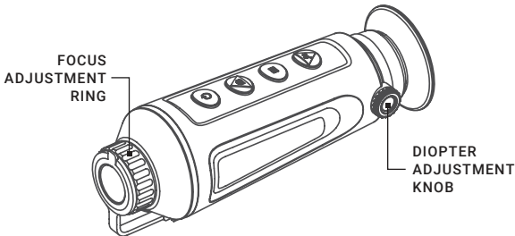
FIGURE 2-4. DIOPTRER AND FOCUS ADJUSTMENT
