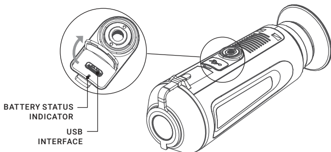
FIGURE 2-1. TAIPAN CHARGING
